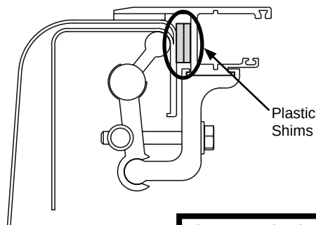
Alternate Style Clamp for certain truck applications
