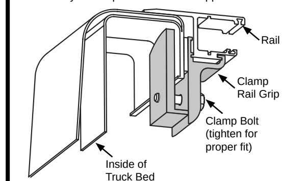
Alternate Style Clamp for certain truck applications
